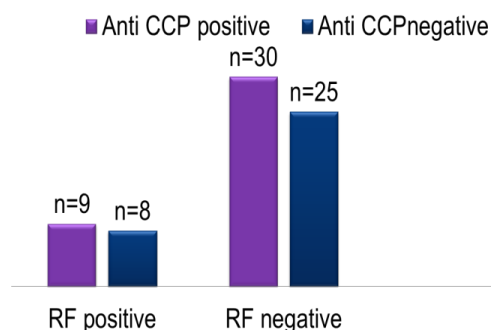
Fig. 3: Comparison of Anti CCP in RF positive and negative samples
