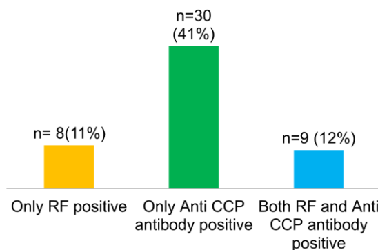
Fig. 1: Comparison of positivity of RF and Anti CCP antibody in clinically suspected RA cases
